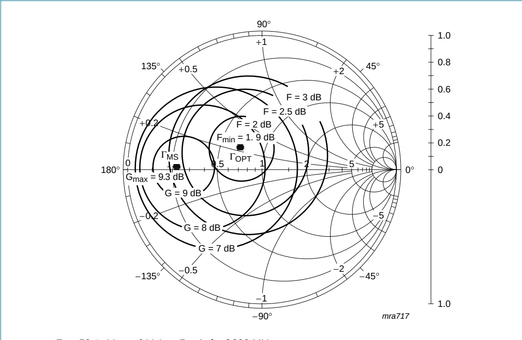
Fig 12. Noise circle figure; f = 2000\text{ MHz} .
